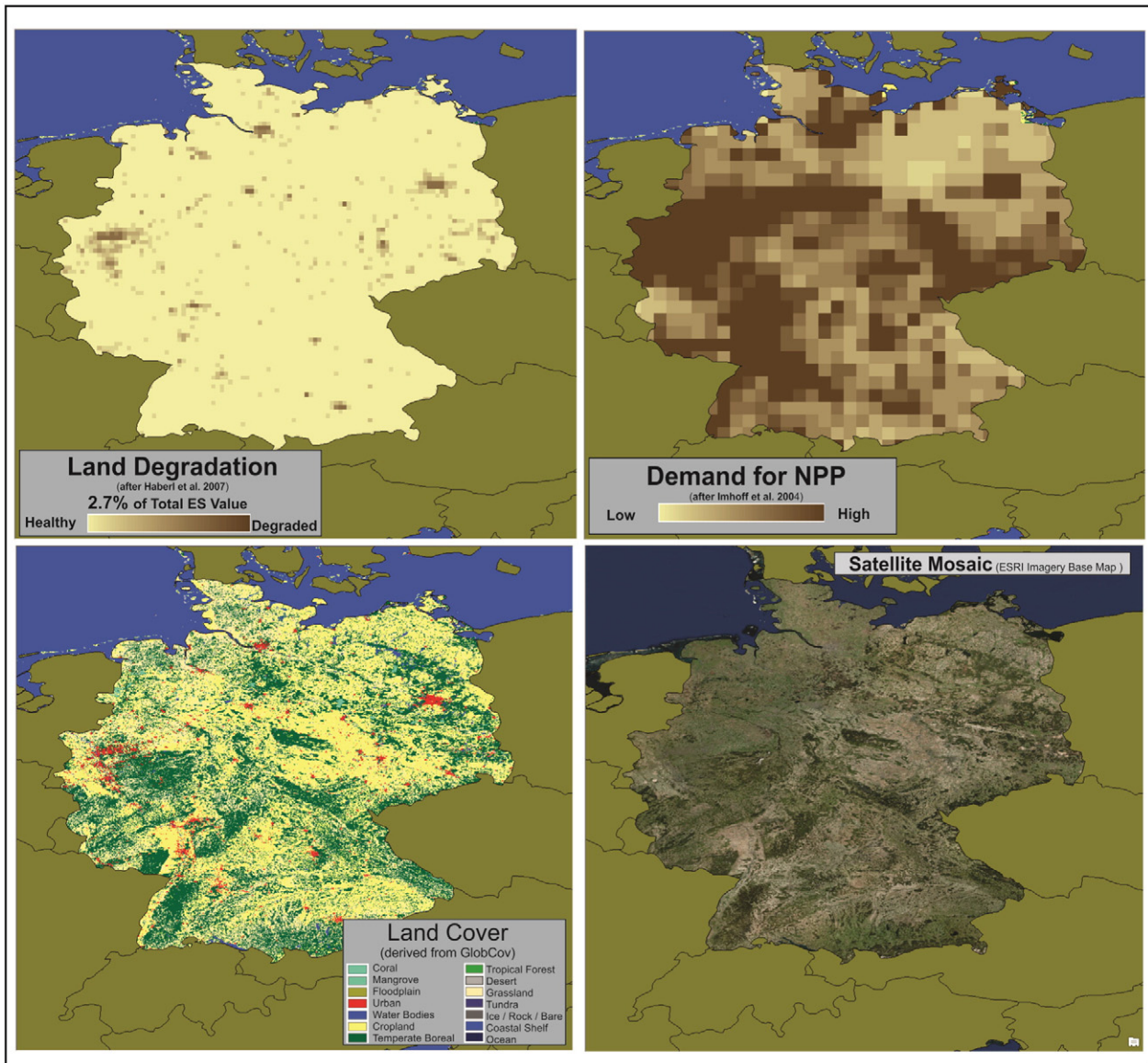
Fig. 6. Representations of land degradation and land cover for Germany.
